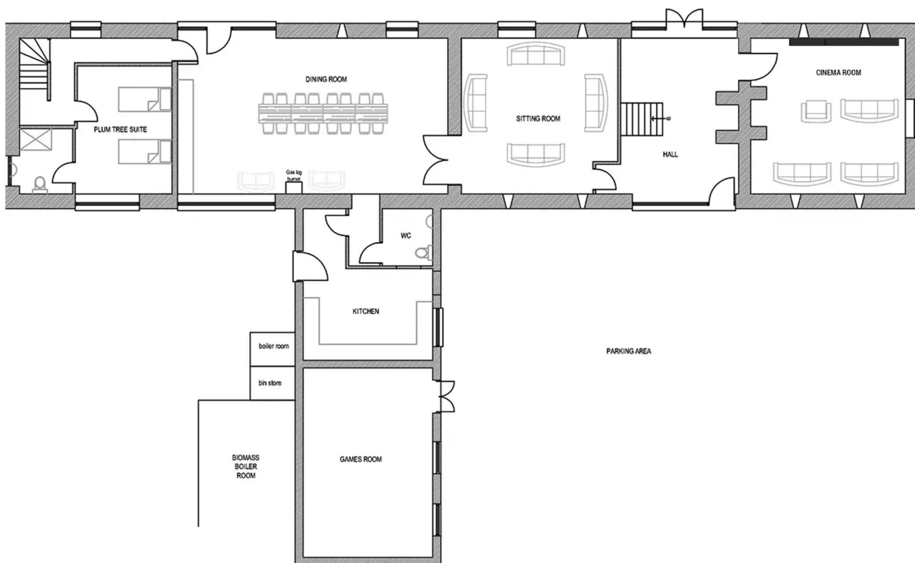
PB Ground Floor
