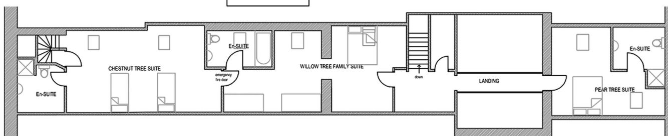
PB Second Floor
